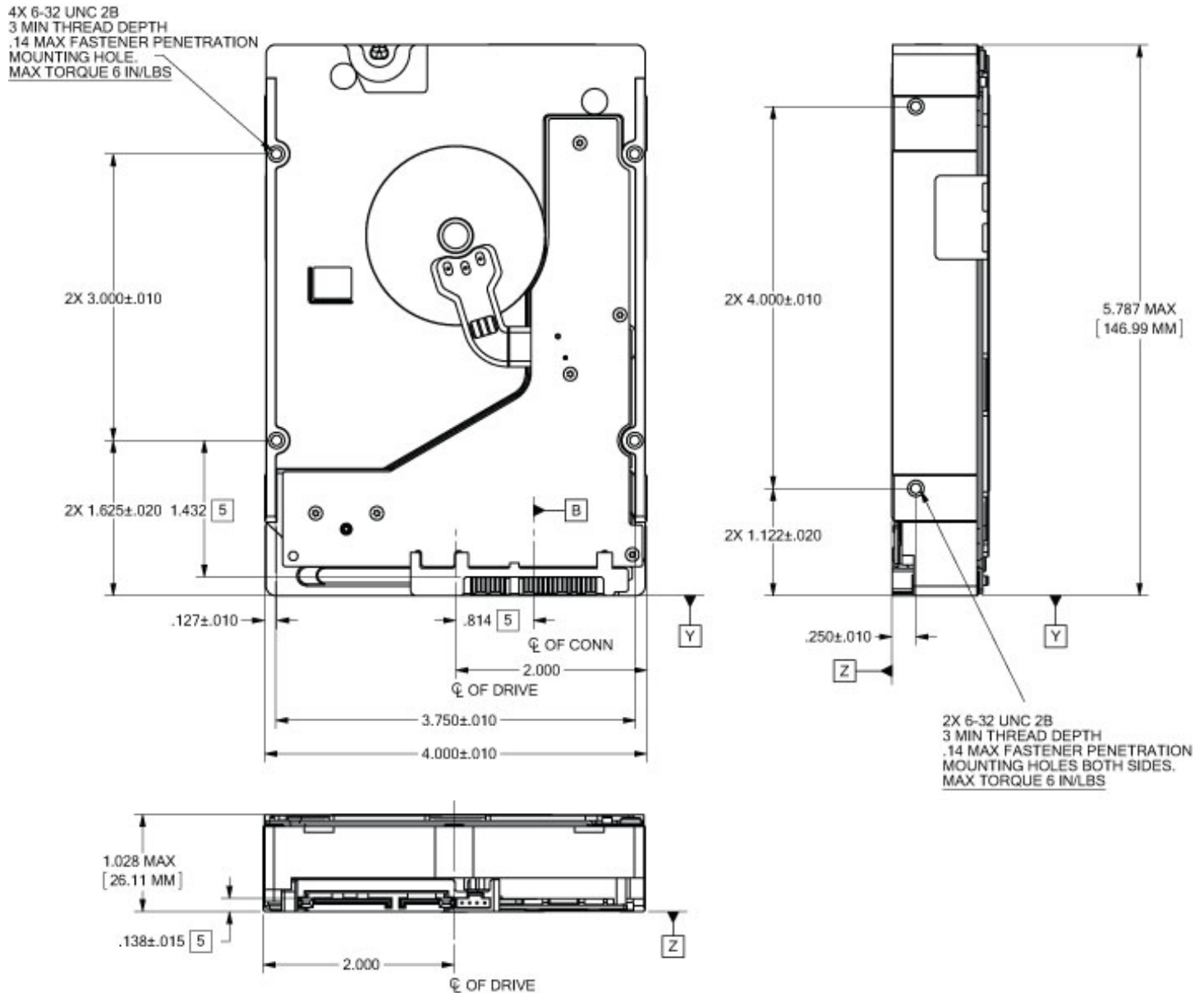
Figure 6. Mounting configuration dimensions (8TB and 6TB models)
