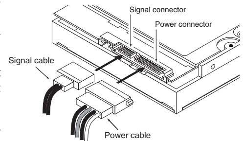
Figure 4. Attaching SATA cabling
